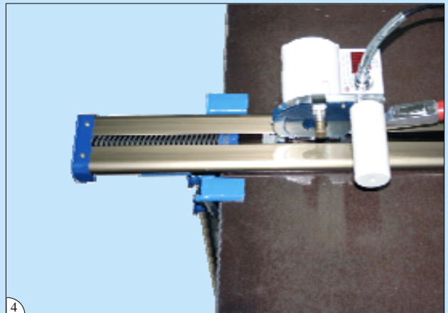
4 回彈裝置 Rebounding device
