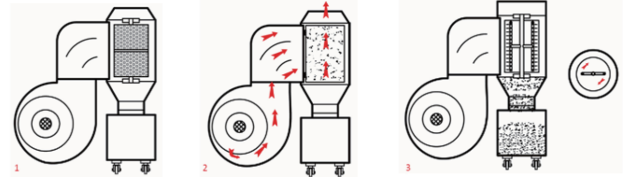
自動環保除塵過濾系統工作原理 Work principle of environment-friendly automatic de-dusting & filtering system
