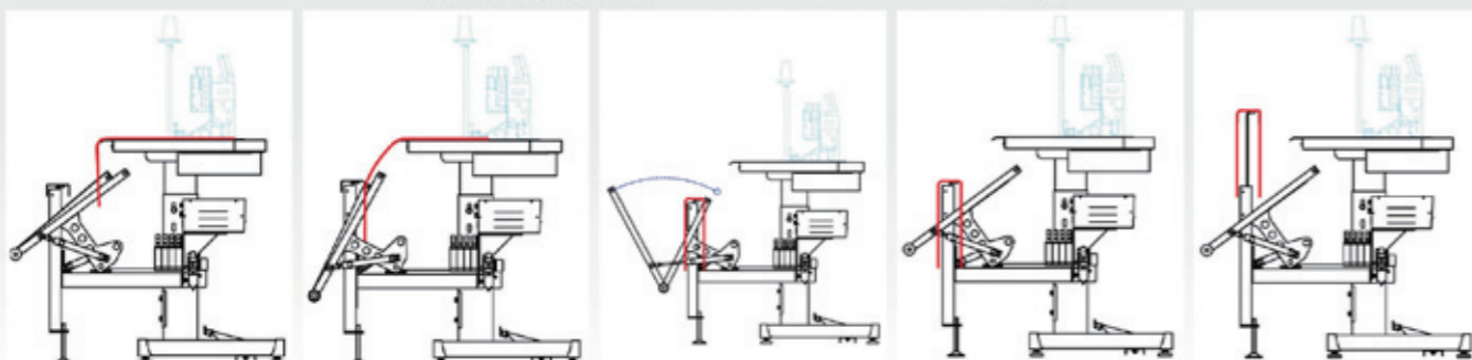
收料架收料流程圖 Flow chart of material stacking
