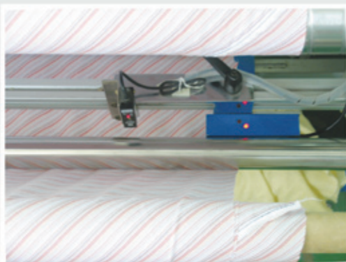
NS-1121對邊感測器/缺料感測器 Edge sensor/no cloth detector
