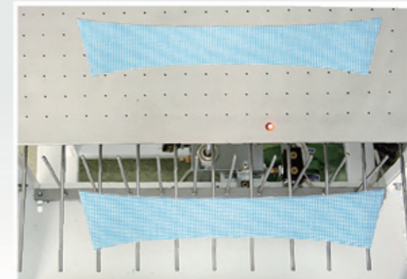
NS-88P 左收料架，自動收、疊料 Left stacker for collecting and stacking material automatically
