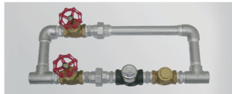
疏水閥總承(管徑規格: 1/2", 1") Steam trap set(pipe diameter :1/2", 1")
