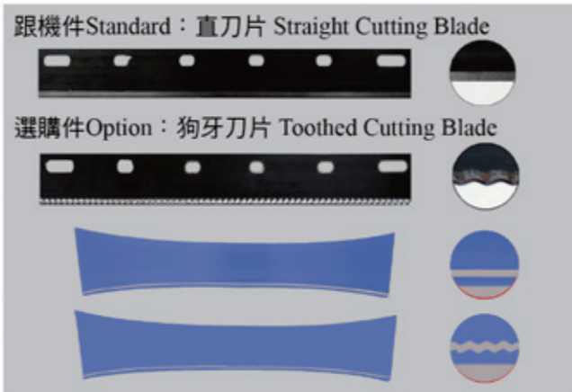
跟機件Standard：直刀片 Straight Cutting Blade 選購件Option：狗牙刀片 Toothed Cutting Blade 修領效果 Collar trimming result
