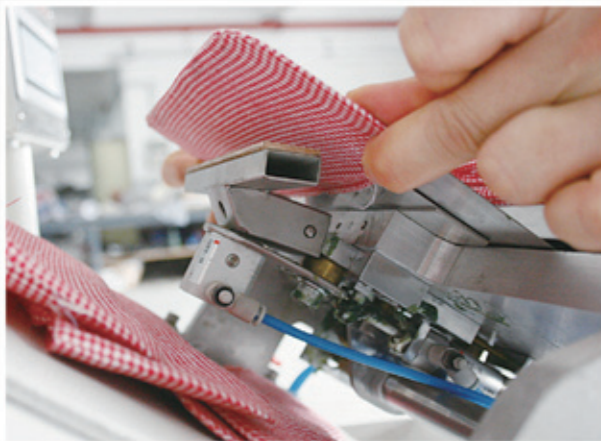
NS-85P自動底夾，防止操作時袖口移位 Automatic bottom clamp for avoiding cuff shift during operation
