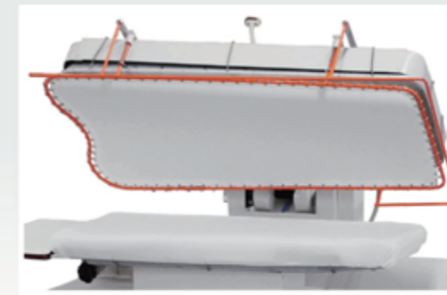
NS-8218AV/NS-8318AV 特設熨布架 Special fabric pre-holding frame
