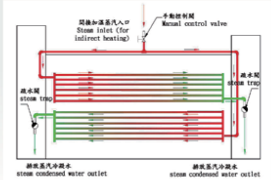
蒸汽間接加溫示意圖 Indirect Steam Heating Diagram
