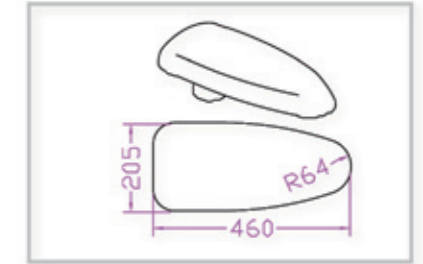
T-A 褲頭熨架 Trousers Topper Buck A
