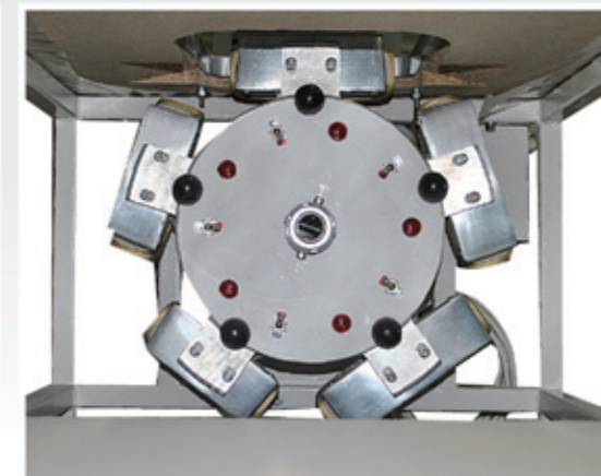
NS-50 可轉動機頭，備有5個不同尺寸模 Rotary head equipped with 5 different sized pressing mould
