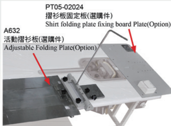
以上兩款需配合使用 The above two types should work with each other
