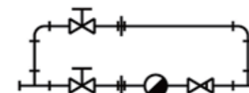
疏水閥總承(管徑規格: 1/2", 1") Steam trap set(pipe diameter :1/2", 1")
