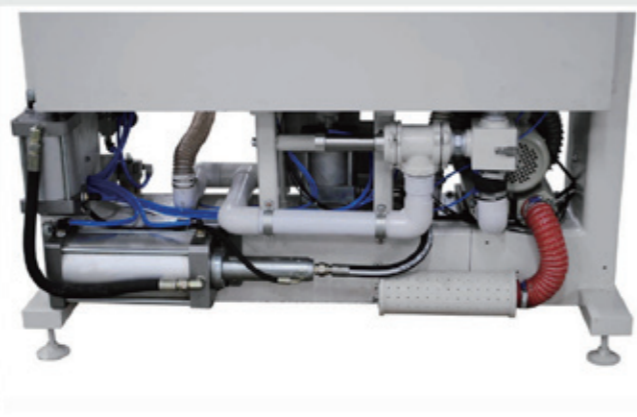
增壓系統 Pressure boosting system
