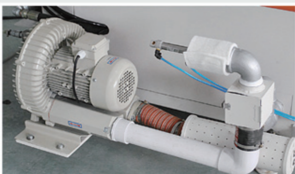
獨立抽風泵 Equipped with independent vacuum pump
