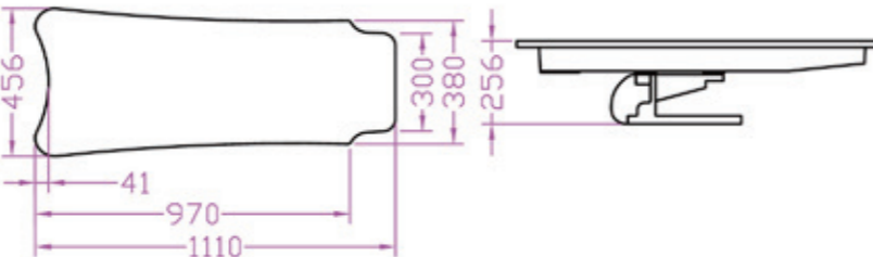
下模尺寸簡圖 Lower mould size (NS-8218, NS-8318, NS-8218P, NS-8318P, NS-8218AV & NS-8318AV)
