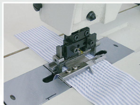
NS-94-1/NS-94AC-1專用於前胸筒對中線用 Designed for matching center line of shirt placket
